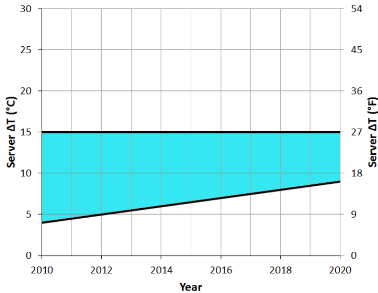
Figure 8 Server \Delta T projection at 45°C (113°F) server inlet temperature [15].
