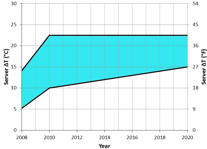
Figure 7 Server \Delta T projection at 35°C (95°F) server inlet temperature [15].
