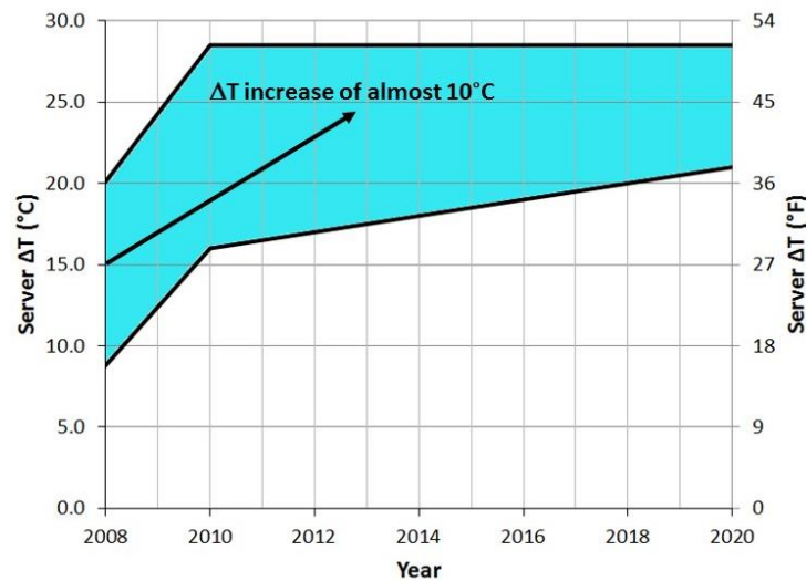
Figure 6 Server \Delta T projection at 25°C (77°F) server inlet temperature [15].
