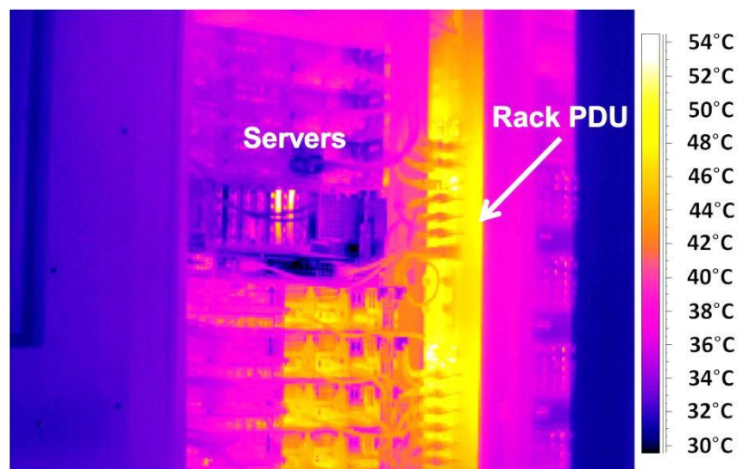
Figure 28 Close-up infrared photo of rack PDU showing internal heat generation.
