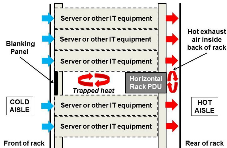
Figure 29 Side view of rack showing heat build-up around installation of a horizontal rack PDU.
