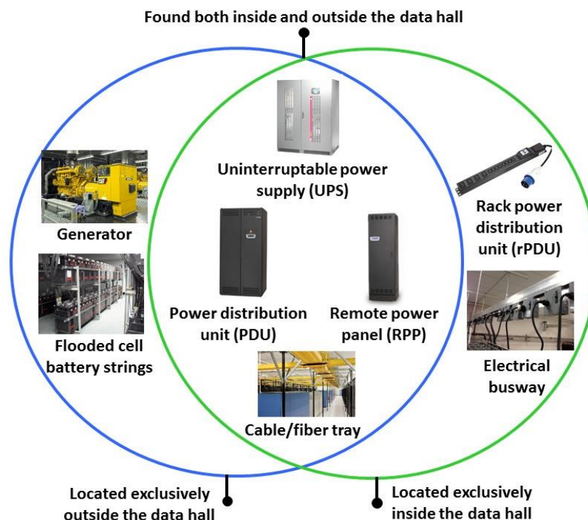
Figure 3 Venn diagram illustrating the physical location of data center power equipment.
