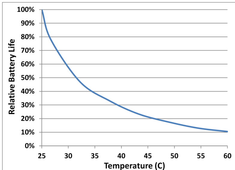
Figure 18 Typical lifetime of a lead-acid battery as a function of temperature. Note that 25°C (77°F) is a typical temperature for 100% of the battery manufacturer's rated lifetime.
