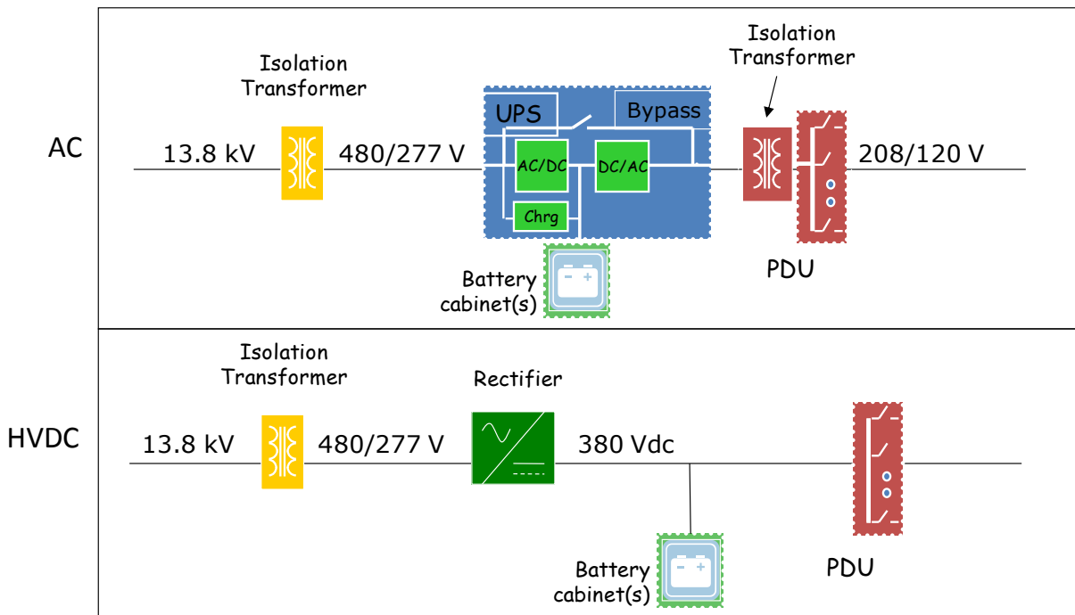
Figure 32 AC and HVDC Power Trains
