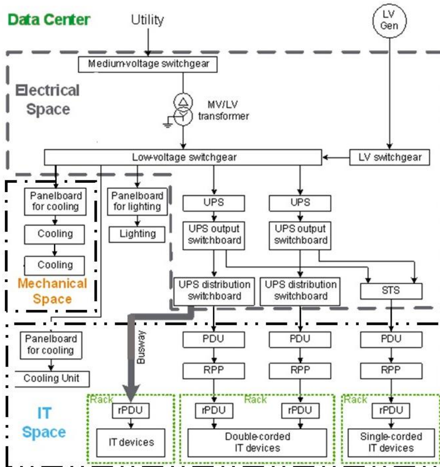
Figure 1 Overview of a typical data center power distribution system [2]. Used with permission.
