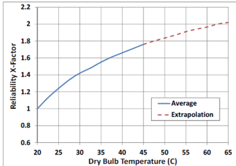
Figure 27 Server reliability x-factor as a function of inlet air temperature (data from [1]).
