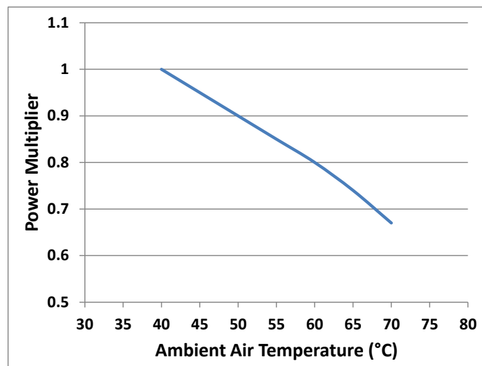
Figure 9 Example of power multipliers showing how power is de-rated (reduced) at ambient air temperatures above the full power capacity rating of 40°C (104°F).
