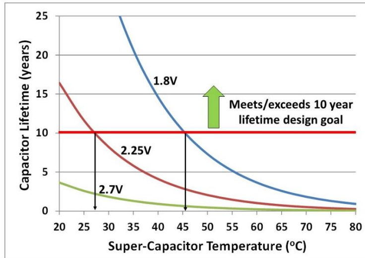
Figure 17 Illustration of lifetime de-rating trade-offs to meet a 10 year design goal for a super-capacitor with a 1,000 hour rating at 70°C (158°F) and 2.7V [24].
