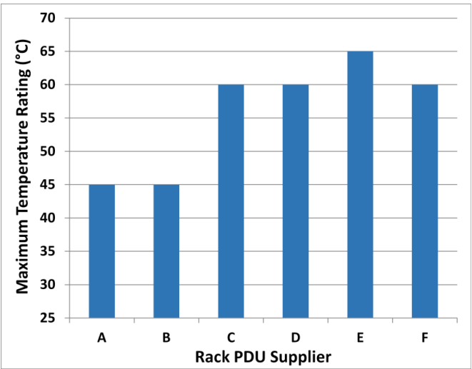
Figure 26 Benchmarking of rack PDU maximum temperature ratings across multiple suppliers.
