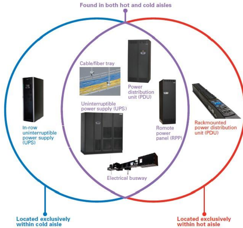
Figure 4 Venn diagram of power equipment located within the data hall (IT equipment space).
